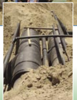
(Top) ISCO technician fuses 36" HDPE pipe in-ditch for a tie-in to an existing line. (Right) HDPE's flexibility allows for multiple pipelines and sizes to be buried together for various applications. The monolithic joints provide a leak-free system.
