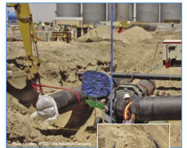
(Top) ISCO technician fuses 36" HDPE pipe in-ditch for a tie-in to an existing line. (Right) HDPE's flexibility allows for multiple pipelines and sizes to be buried together for various applications. The monolithic joints provide a leak-free system.
